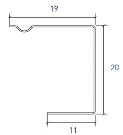
C SECTION
